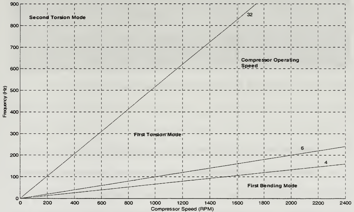
Figure 4.4 Rotor Blade Campbell Diagram.
